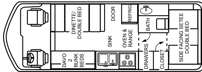
FLOOR PLAN 26'-3
