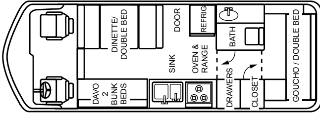
FLOOR PLAN 26'-2
