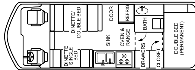
FLOOR PLAN 26'-4
