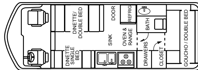
FLOOR PLAN 26'-5
