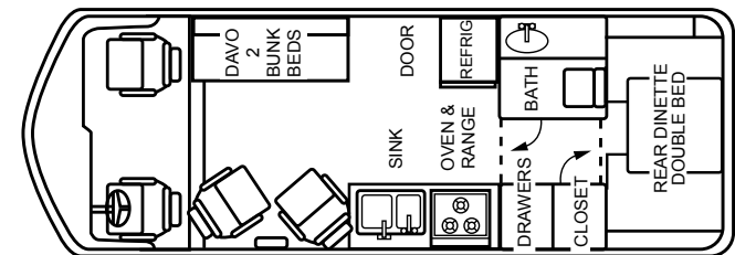
FLOOR PLAN 26'-11
