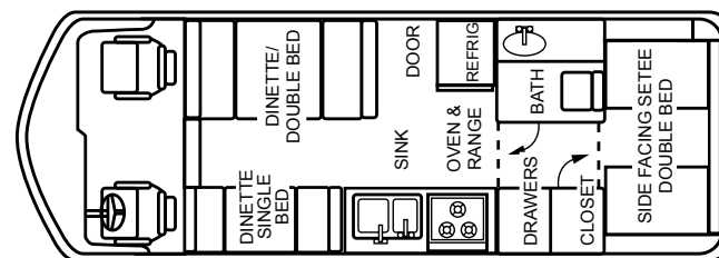
FLOOR PLAN 26'-6
