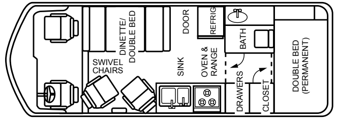
BASE FLOOR PLAN 26'-7
