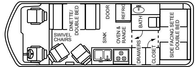
FLOOR PLAN 26'-9
