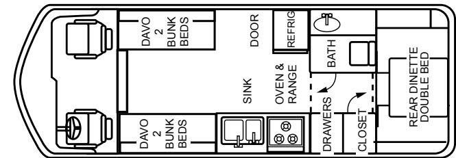
FLOOR PLAN 26'-10
