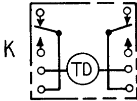
Relay with D.P.D.T. contacts
