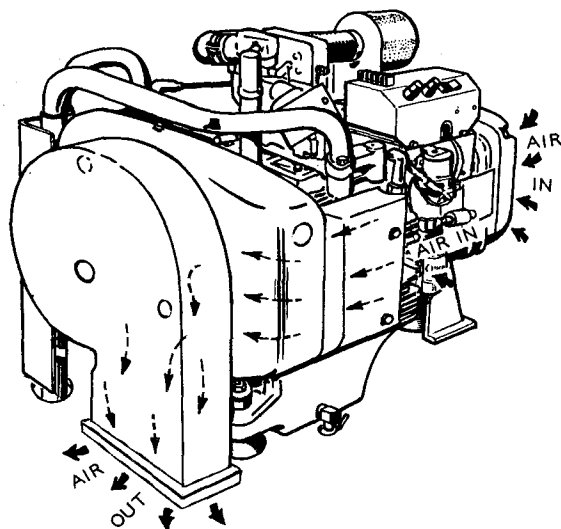
FIGURE 4. TYPICAL ONAN RV COOLING SYSTEM
