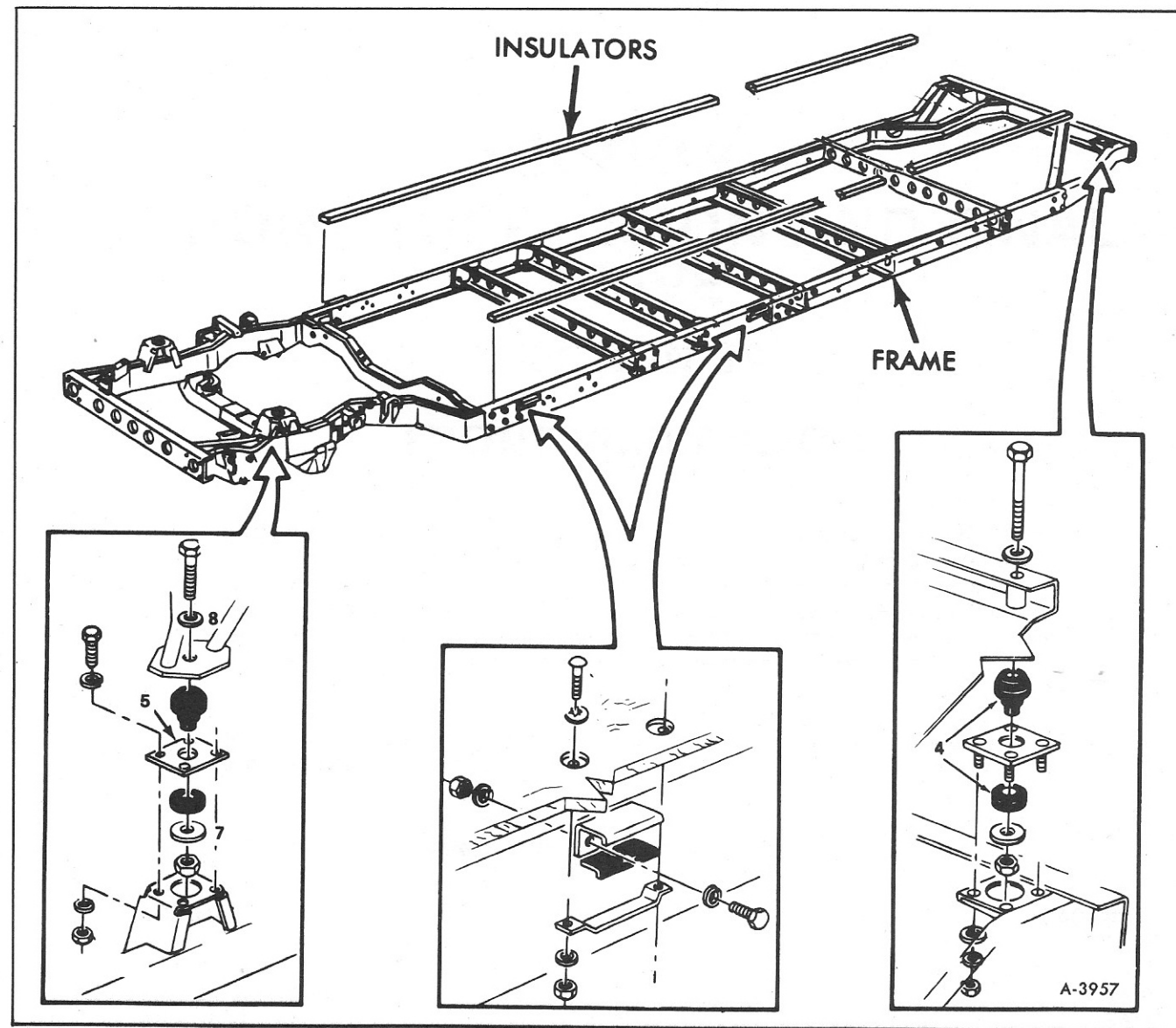
Figure 4—Body Mountings
