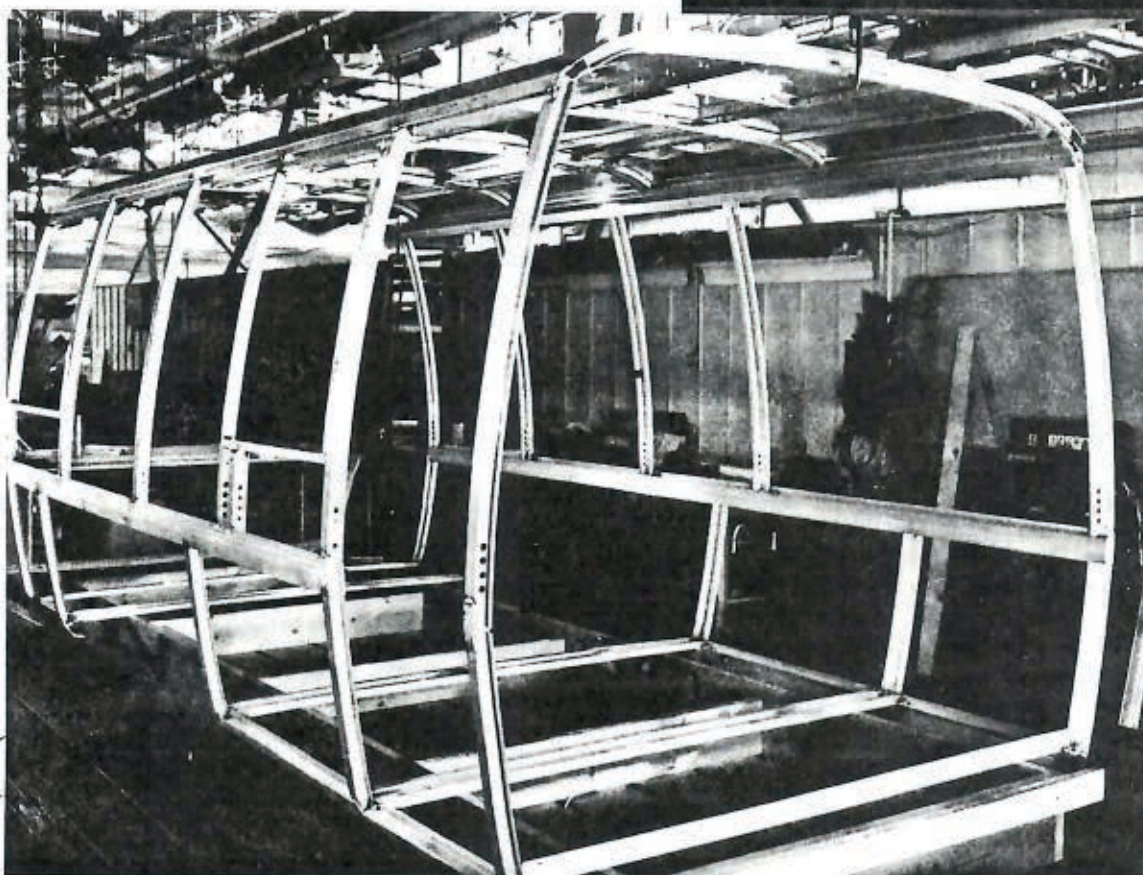
FRAMING CONSTRUCTION
